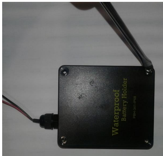
Fig. 20 – Unscrewing battery box
