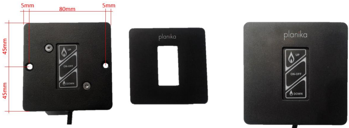
Fig. 17 – Location of mounting holes and magnetic sticker
