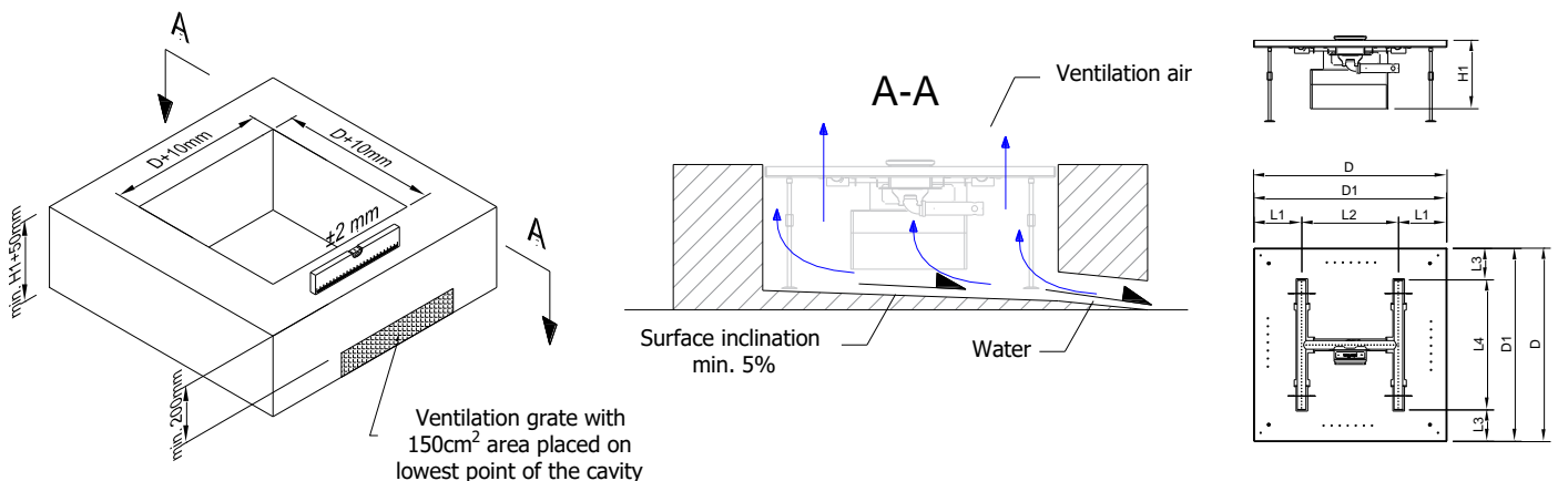
Fig 3 – Cavity size
